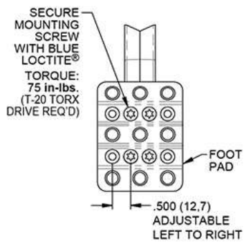
FOOT PAD DETAIL
